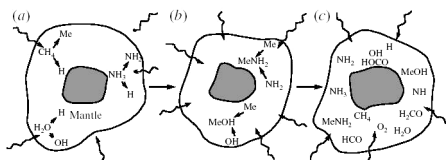
Figure 2. Structure of grains when they initially accrete is inferred from laboratory simulations in which mixtures of water, methane, ammonia and other simple molecules are subjected to ultraviolet irradiation at a temperature of 10 K. Each grain begins as a silicate core that condensed in the atmosphere of a cool giant star. Around this core a mantle of ice forms. Ultraviolet radiation breaks some of the mantle molecules into radicals, or reactive molecular fragments (a). The radicals can then recombine in new ways (b). Over a longer period the continued ultraviolet irradiation of the grain can give rise to ever more complex mixtures of molecules and radicals (c). 1
