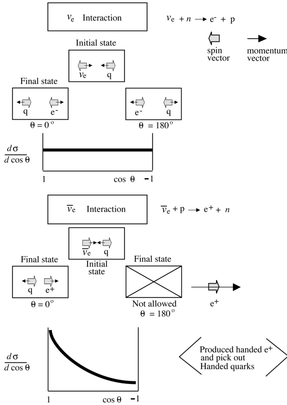
Figure 1. (b) Example of handedness in the weak interaction
