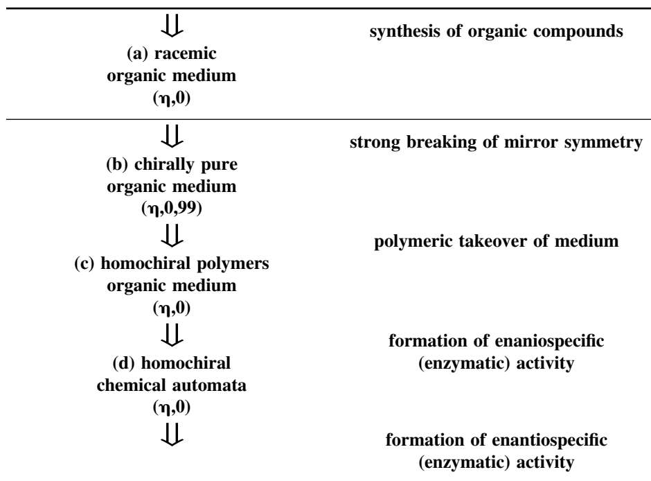
Figure 5. Five main stages of prebiological evolution.
