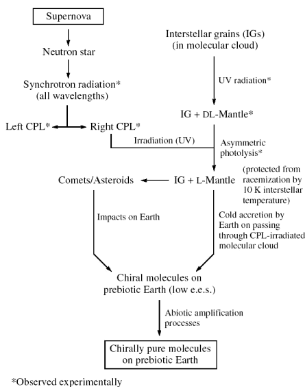
Figure 4. Possible extraterrestrial origin of terrestrial homochirality. 1,3
