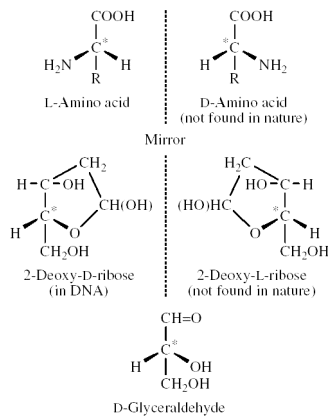
Figure 1. (a) Examples of molecules that are isomers, some of which exist in nature and some that do not.
