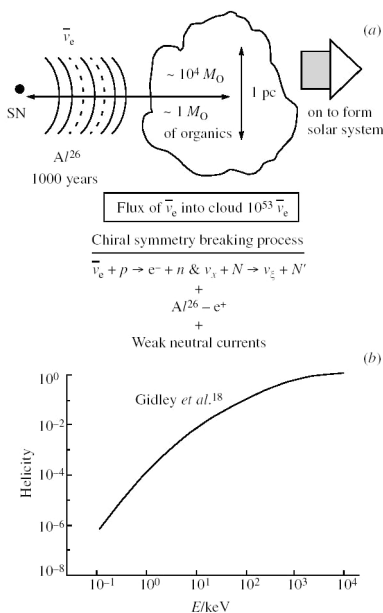
Figure 3. (A) Schematic of the effect of a supernova II on the organic molecules in a dense molecular cloud. (B) Estimated polarization of the \beta^* decay particles as the energy decreases by ionization in \text{H}_2\text{O} and in the dense molecular cloud. One observation of the polarization of low energy e^* by the Michigan group. 1
